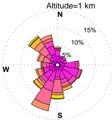
WINDROSES. BELTSVILLE, MD WIND PROFILER. AUGUST, HOURS: 10 am to 7 pm YEAR: 2014
