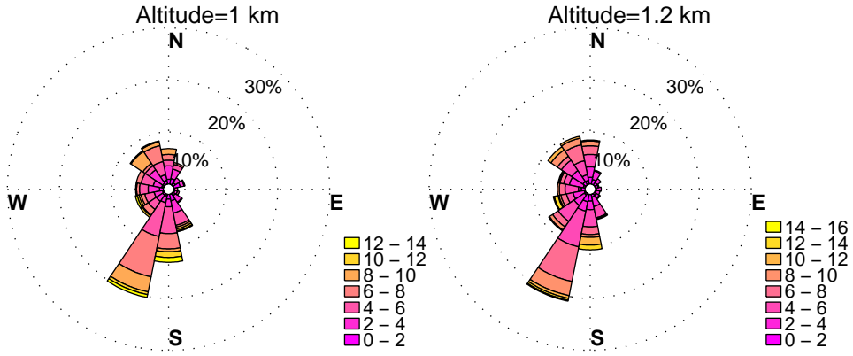
WINDROSES. BELTSVILLE, MD WIND PROFILER. JUNE, HOURS: 10 am to 7 pm YEAR: 2014
