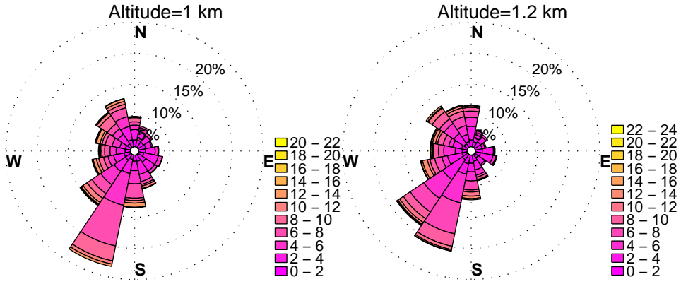
WINDROSES. BELTSVILLE, MD WIND PROFILER. MONTHS: JUNE to AUGUST, HOURS: 10 am to 7 pm YEAR: 2014
