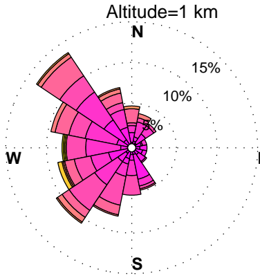
WINDROSES. BELTSVILLE, MD WIND PROFILER. JULY, HOURS: 10 am to 7 pm YEAR: 2015
