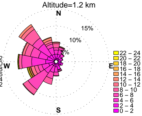
WINDROSES. BELTSVILLE, MD WIND PROFILER. JULY, HOURS: 10 am to 7 pm YEAR: 2015
