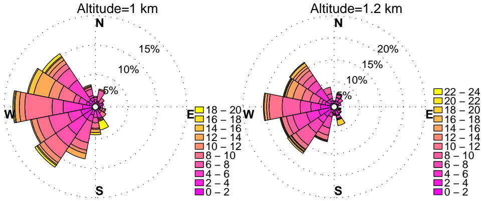
WINDROSES. BELTSVILLE, MD WIND PROFILER. JUNE, HOURS: 10 am to 7 pm YEAR: 2015
