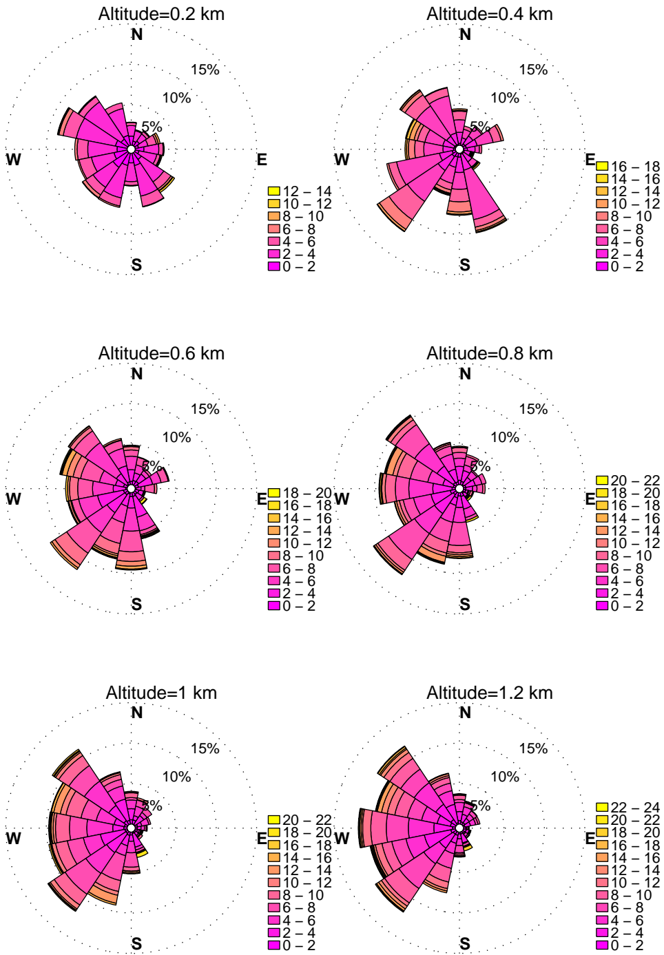
WINDROSES. BELTSVILLE, MD WIND PROFILER. MONTHS: JUNE to AUGUST, HOURS: 10 am to 7 pm YEAR: 2015
