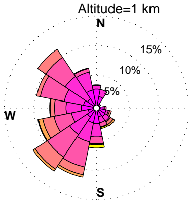
WINDROSES. BELTSVILLE, MD WIND PROFILER. APRIL, HOURS: 12 pm to 3 pm DATA: FROM 2010 to 2015
