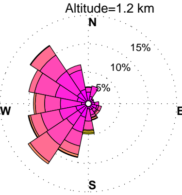
WINDROSES. BELTSVILLE, MD WIND PROFILER. APRIL, HOURS: 12 pm to 3 pm DATA: FROM 2010 to 2015
