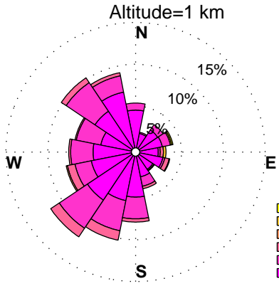
WINDROSES. BELTSVILLE, MD WIND PROFILER. AUGUST, HOURS: 12 pm to 3 pm DATA: FROM 2010 to 2015
