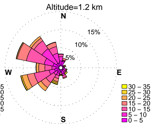
WINDROSES. BELTSVILLE, MD WIND PROFILER. DECEMBER, HOURS: 12 pm to 3 pm DATA: FROM 2010 to 2015
