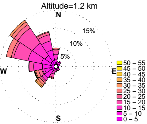
WINDROSES. BELTSVILLE, MD WIND PROFILER. FEBRUARY, HOURS: 12 am to 3 am DATA: FROM 2010 to 2015
