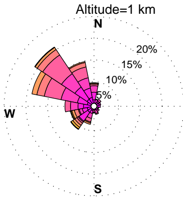
WINDROSES. BELTSVILLE, MD WIND PROFILER. FEBRUARY, HOURS: 12 am to 3 am DATA: FROM 2010 to 2015
