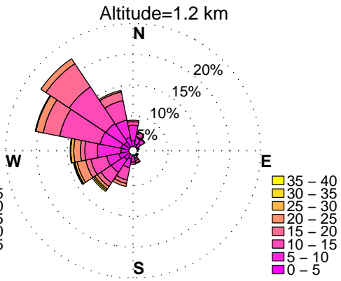
WINDROSES. BELTSVILLE, MD WIND PROFILER. FEBRUARY, HOURS: 12 pm to 3 pm DATA: FROM 2010 to 2015
