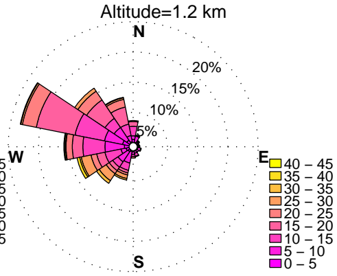
WINDROSES. BELTSVILLE, MD WIND PROFILER. JANUARY, HOURS: 12 am to 3 am DATA: FROM 2010 to 2015
