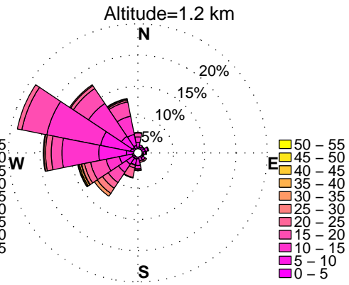
WINDROSES. BELTSVILLE, MD WIND PROFILER. JANUARY, HOURS: 12 pm to 3 pm DATA: FROM 2010 to 2015
