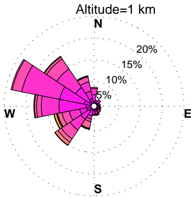
WINDROSES. BELTSVILLE, MD WIND PROFILER. JANUARY, HOURS: 12 pm to 3 pm DATA: FROM 2010 to 2015
