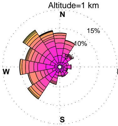
WINDROSES. BELTSVILLE, MD WIND PROFILER. JULY, HOURS: 12 am to 3 am DATA: FROM 2010 to 2015
