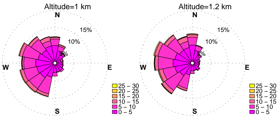
WINDROSES. BELTSVILLE, MD WIND PROFILER. JULY, HOURS: 10 am to 7 pm DATA: FROM 2010 to 2015
