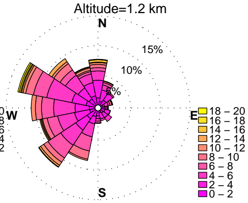
WINDROSES. BELTSVILLE, MD WIND PROFILER. JULY, HOURS: 12 pm to 3 pm DATA: FROM 2010 to 2015
