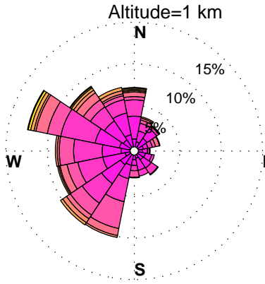
WINDROSES. BELTSVILLE, MD WIND PROFILER. JULY, HOURS: 12 pm to 3 pm DATA: FROM 2010 to 2015
