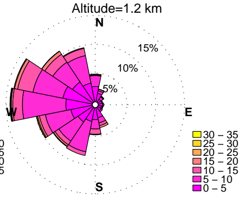
WINDROSES. BELTSVILLE, MD WIND PROFILER. JUNE, HOURS: 10 am to 7 pm DATA: FROM 2010 to 2015
