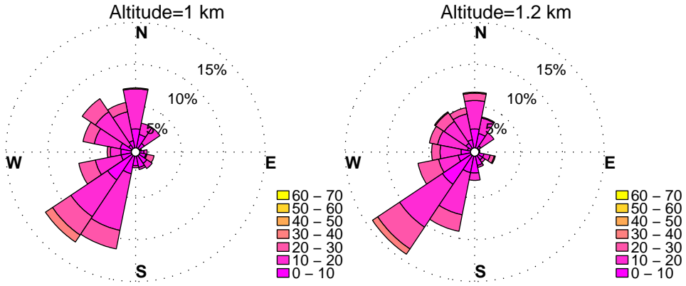
WINDROSES. BELTSVILLE, MD WIND PROFILER. MARCH, HOURS: 12 am to 3 am DATA: FROM 2010 to 2015
