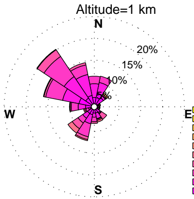
WINDROSES. BELTSVILLE, MD WIND PROFILER. MARCH, HOURS: 12 pm to 3 pm DATA: FROM 2010 to 2015
