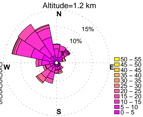
WINDROSES. BELTSVILLE, MD WIND PROFILER. MARCH, HOURS: 12 pm to 3 pm DATA: FROM 2010 to 2015
