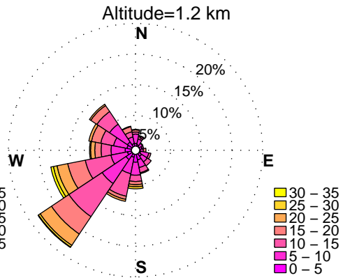
WINDROSES. BELTSVILLE, MD WIND PROFILER. MAY, HOURS: 12 am to 3 am DATA: FROM 2010 to 2015
