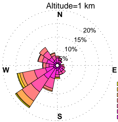
WINDROSES. BELTSVILLE, MD WIND PROFILER. MAY, HOURS: 12 am to 3 am DATA: FROM 2010 to 2015
