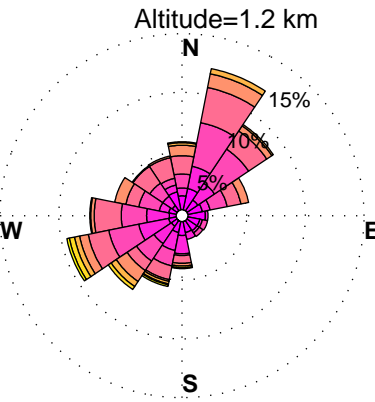
WINDROSES. BELTSVILLE, MD WIND PROFILER. NOVEMBER, HOURS: 12 am to 3 am DATA: FROM 2010 to 2015
