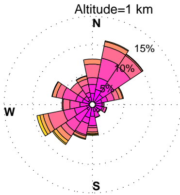
WINDROSES. BELTSVILLE, MD WIND PROFILER. NOVEMBER, HOURS: 12 am to 3 am DATA: FROM 2010 to 2015
