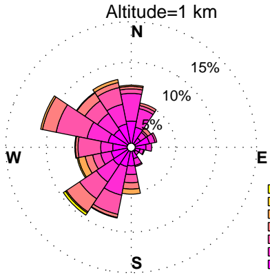
WINDROSES. BELTSVILLE, MD WIND PROFILER. NOVEMBER, HOURS: 12 pm to 3 pm DATA: FROM 2010 to 2015
