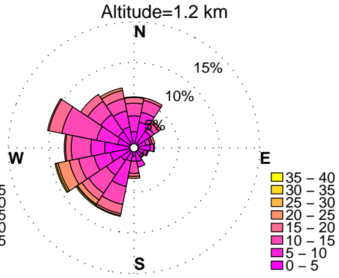
WINDROSES. BELTSVILLE, MD WIND PROFILER. NOVEMBER, HOURS: 12 pm to 3 pm DATA: FROM 2010 to 2015
