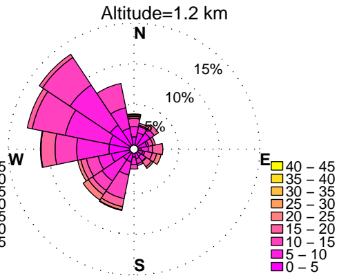
WINDROSES. BELTSVILLE, MD WIND PROFILER. OCTOBER, HOURS: 12 pm to 3 pm DATA: FROM 2010 to 2015
