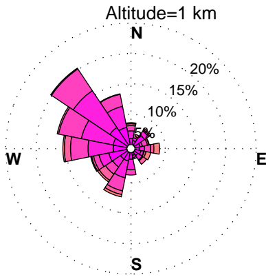
WINDROSES. BELTSVILLE, MD WIND PROFILER. OCTOBER, HOURS: 12 pm to 3 pm DATA: FROM 2010 to 2015
