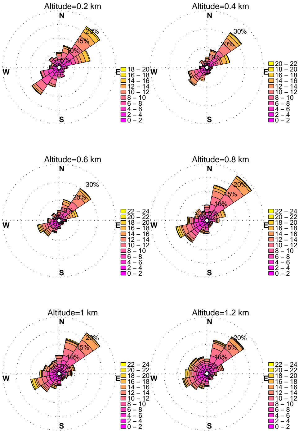
WINDROSES. BELTSVILLE, MD WIND PROFILER. SEPTEMBER, HOURS: 12 am to 3 am DATA: FROM 2010 to 2015
