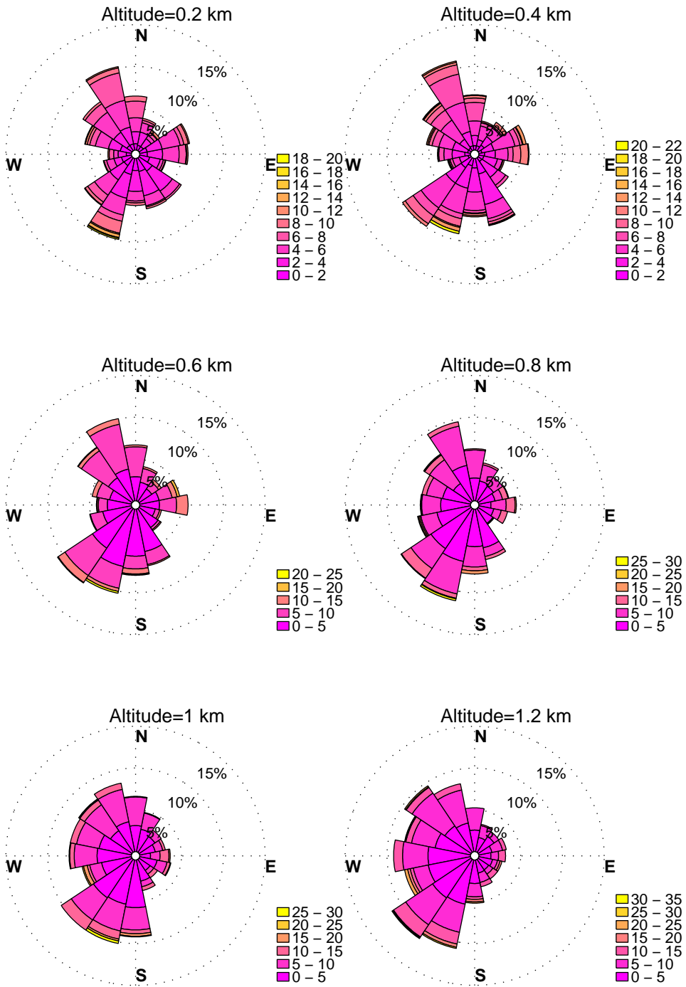
WINDROSES. BELTSVILLE, MD WIND PROFILER. SEPTEMBER, HOURS: 12 pm to 3 pm DATA: FROM 2010 to 2015
