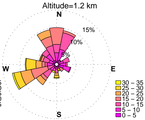
WINDROSES. HORN POINT, MD WIND PROFILER. APRIL, HOURS: 12 am to 3 am DATA: FROM 6/2012 to 12/2015
