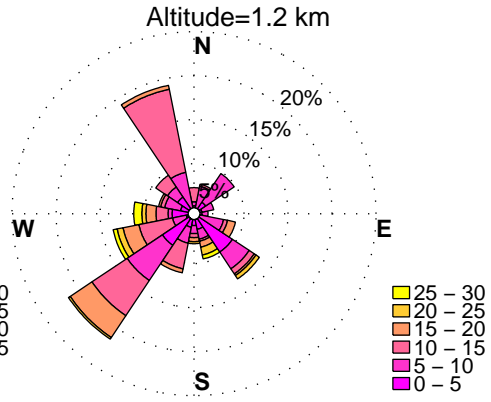
WINDROSES. HORN POINT, MD WIND PROFILER. APRIL, HOURS: 12 pm to 3 pm DATA: FROM 6/2012 to 12/2015
