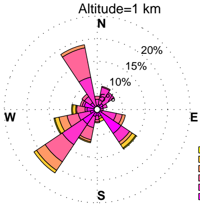
WINDROSES. HORN POINT, MD WIND PROFILER. APRIL, HOURS: 12 pm to 3 pm DATA: FROM 6/2012 to 12/2015
