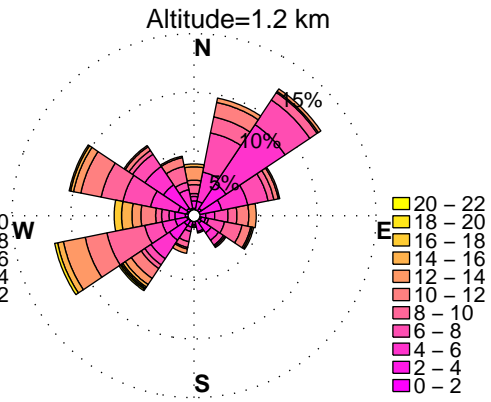
WINDROSES. HORN POINT, MD WIND PROFILER. AUGUST, HOURS: 12 am to 3 am DATA: FROM 6/2012 to 12/2015
