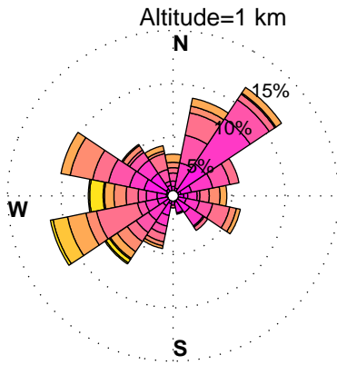
WINDROSES. HORN POINT, MD WIND PROFILER. AUGUST, HOURS: 12 am to 3 am DATA: FROM 6/2012 to 12/2015
