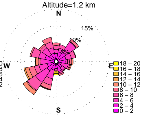
WINDROSES. HORN POINT, MD WIND PROFILER. AUGUST, HOURS: 12 pm to 3 pm DATA: FROM 6/2012 to 12/2015
