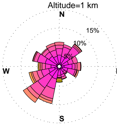
WINDROSES. HORN POINT, MD WIND PROFILER. AUGUST, HOURS: 12 pm to 3 pm DATA: FROM 6/2012 to 12/2015
