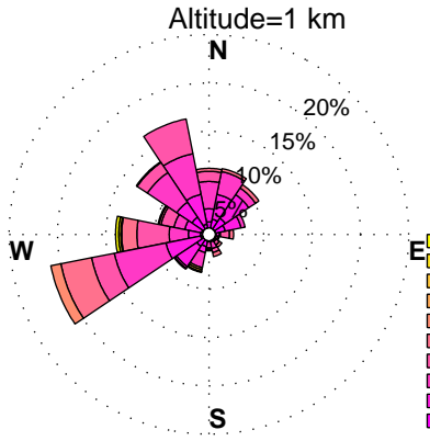
WINDROSES. HORN POINT, MD WIND PROFILER. DECEMBER, HOURS: 12 am to 3 am DATA: FROM 6/2012 to 12/2015
