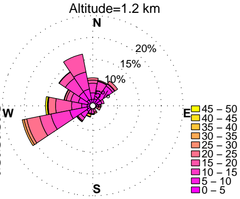
WINDROSES. HORN POINT, MD WIND PROFILER. DECEMBER, HOURS: 12 am to 3 am DATA: FROM 6/2012 to 12/2015
