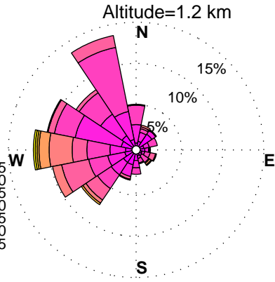
WINDROSES. HORN POINT, MD WIND PROFILER. DECEMBER, HOURS: 12 pm to 3 pm DATA: FROM 6/2012 to 12/2015
