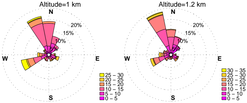
WINDROSES. HORN POINT, MD WIND PROFILER. FEBRUARY, HOURS: 12 am to 3 am DATA: FROM 6/2012 to 12/2015
