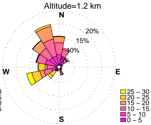
WINDROSES. HORN POINT, MD WIND PROFILER. JANUARY, HOURS: 12 am to 3 am DATA: FROM 6/2012 to 12/2015
