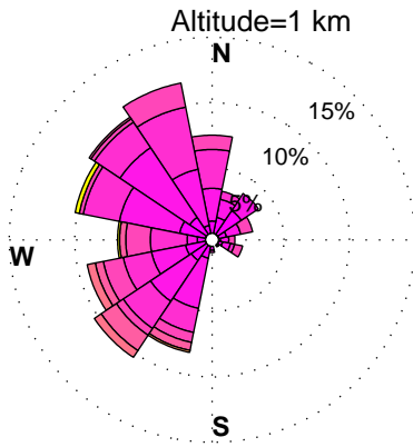
WINDROSES. HORN POINT, MD WIND PROFILER. JANUARY, HOURS: 12 pm to 3 pm DATA: FROM 6/2012 to 12/2015
