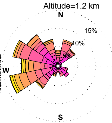
WINDROSES. HORN POINT, MD WIND PROFILER. JUNE, HOURS: 12 am to 3 am DATA: FROM 6/2012 to 12/2015
