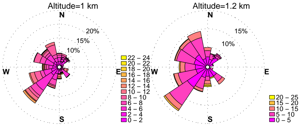
WINDROSES. HORN POINT, MD WIND PROFILER. JUNE, HOURS: 12 pm to 3 pm DATA: FROM 6/2012 to 12/2015
