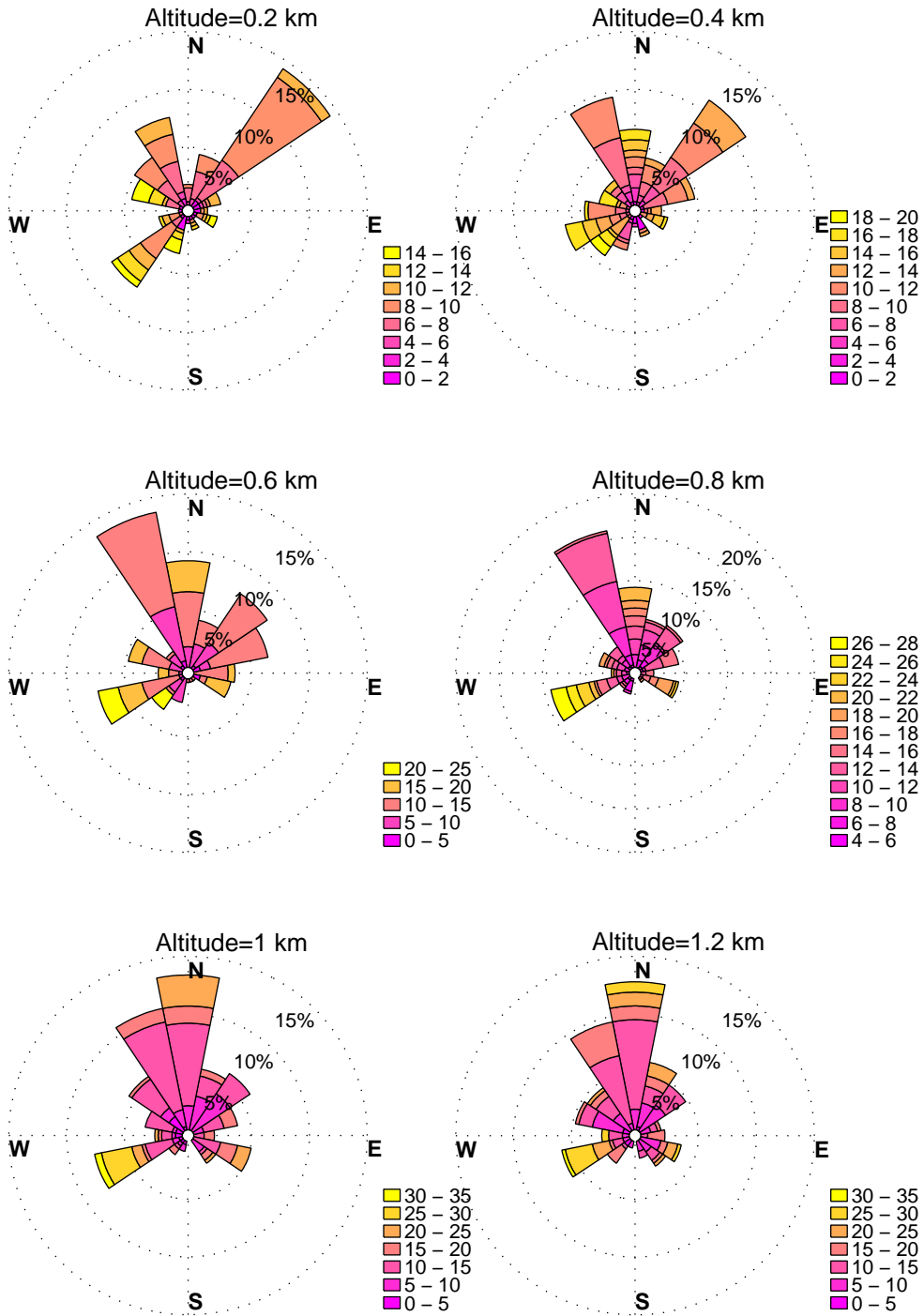
WINDROSES. HORN POINT, MD WIND PROFILER. MARCH, HOURS: 12 am to 3 am DATA: FROM 6/2012 to 12/2015
