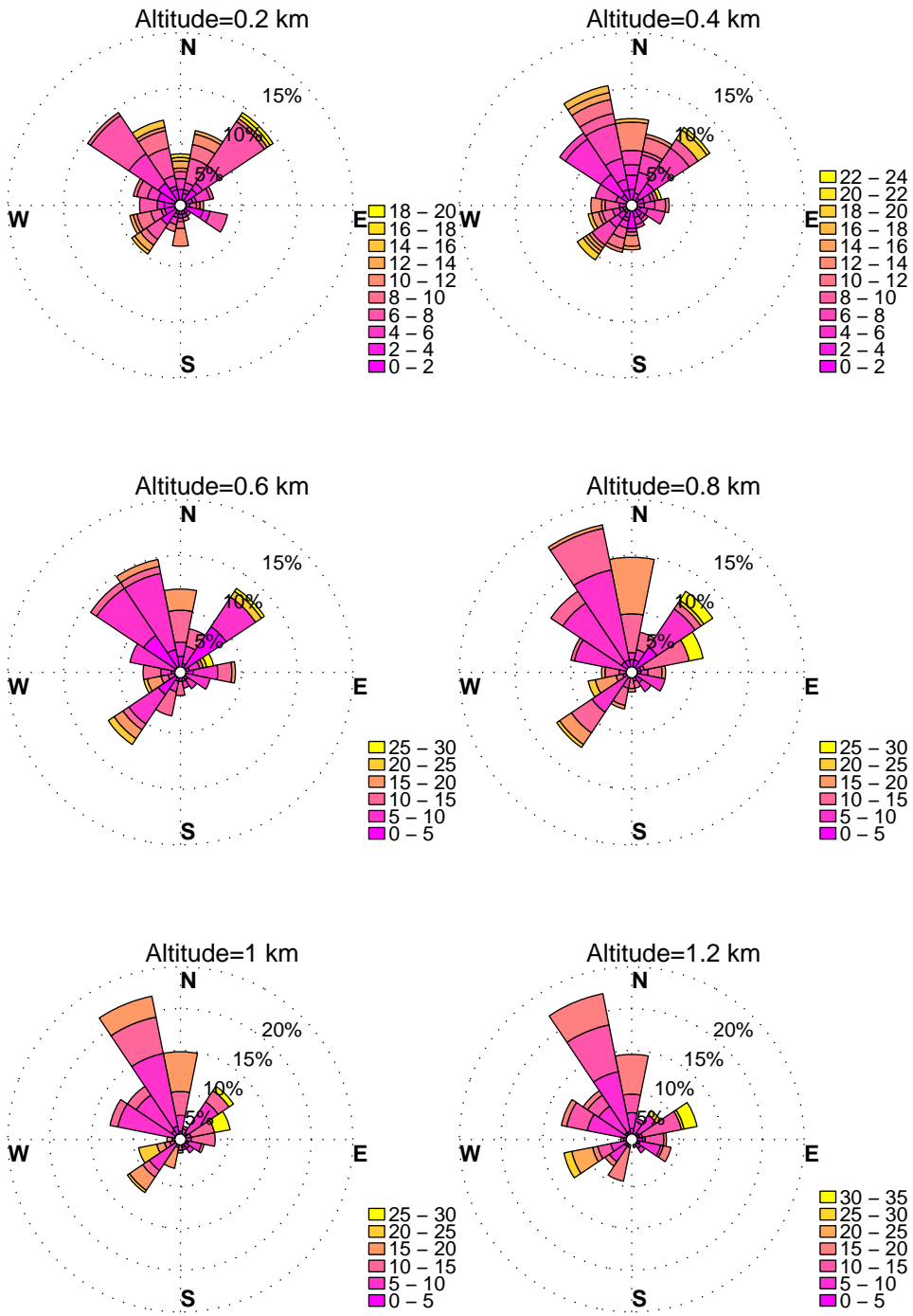
WINDROSES. HORN POINT, MD WIND PROFILER. MARCH, HOURS: 12 pm to 3 pm DATA: FROM 6/2012 to 12/2015
