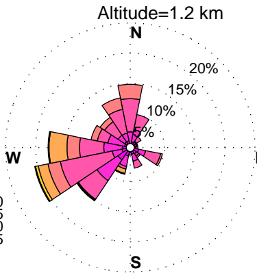
WINDROSES. HORN POINT, MD WIND PROFILER. MAY, HOURS: 12 am to 3 am DATA: FROM 6/2012 to 12/2015
