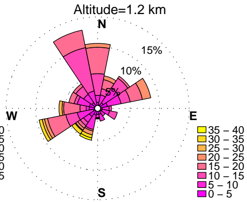
WINDROSES. HORN POINT, MD WIND PROFILER. NOVEMBER, HOURS: 12 am to 3 am DATA: FROM 6/2012 to 12/2015
