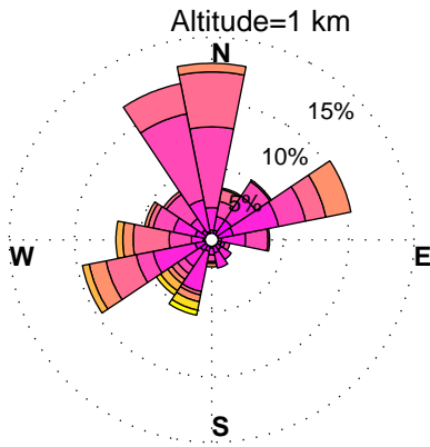
WINDROSES. HORN POINT, MD WIND PROFILER. NOVEMBER, HOURS: 12 am to 3 am DATA: FROM 6/2012 to 12/2015
