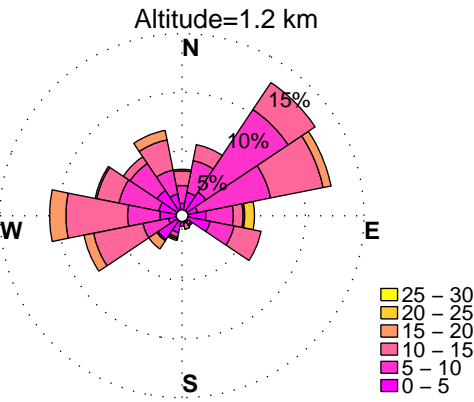
WINDROSES. HORN POINT, MD WIND PROFILER. SEPTEMBER, HOURS: 12 am to 3 am DATA: FROM 6/2012 to 12/2015
