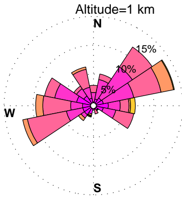
WINDROSES. HORN POINT, MD WIND PROFILER. SEPTEMBER, HOURS: 12 am to 3 am DATA: FROM 6/2012 to 12/2015
