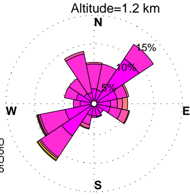
WINDROSES. HORN POINT, MD WIND PROFILER. SEPTEMBER, HOURS: 12 pm to 3 pm DATA: FROM 6/2012 to 12/2015
