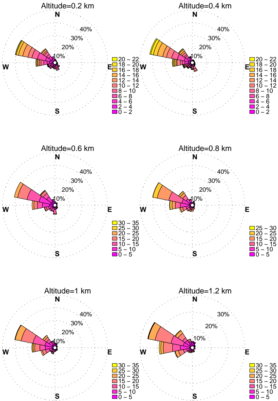
WINDROSES. PINEY RUN, MD WIND PROFILER. FEBRUARY, HOURS: 12 pm to 15 pm DATA: FROM 1/2010 to 8/2014
