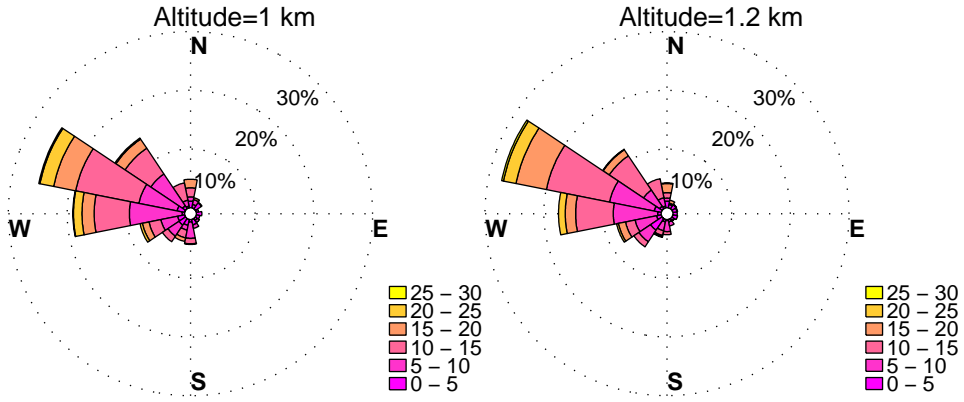
WINDROSES. PINEY RUN, MD WIND PROFILER. JUNE, HOURS: 12 am to 3 am DATA: FROM 1/2010 to 8/2014
