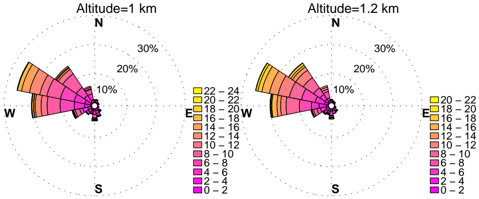
WINDROSES. PINEY RUN, MD WIND PROFILER. JUNE, HOURS: 12 pm to 15 pm DATA: FROM 1/2010 to 8/2014
