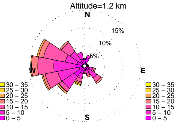
WINDROSES. PINEY RUN, MD WIND PROFILER. MAY, HOURS: 12 pm to 15 pm DATA: FROM 1/2010 to 8/2014
