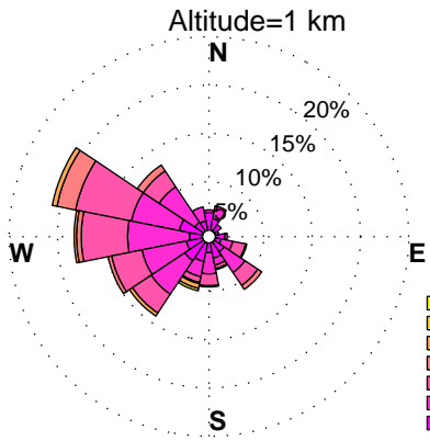
WINDROSES. PINEY RUN, MD WIND PROFILER. MAY, HOURS: 12 pm to 15 pm DATA: FROM 1/2010 to 8/2014
