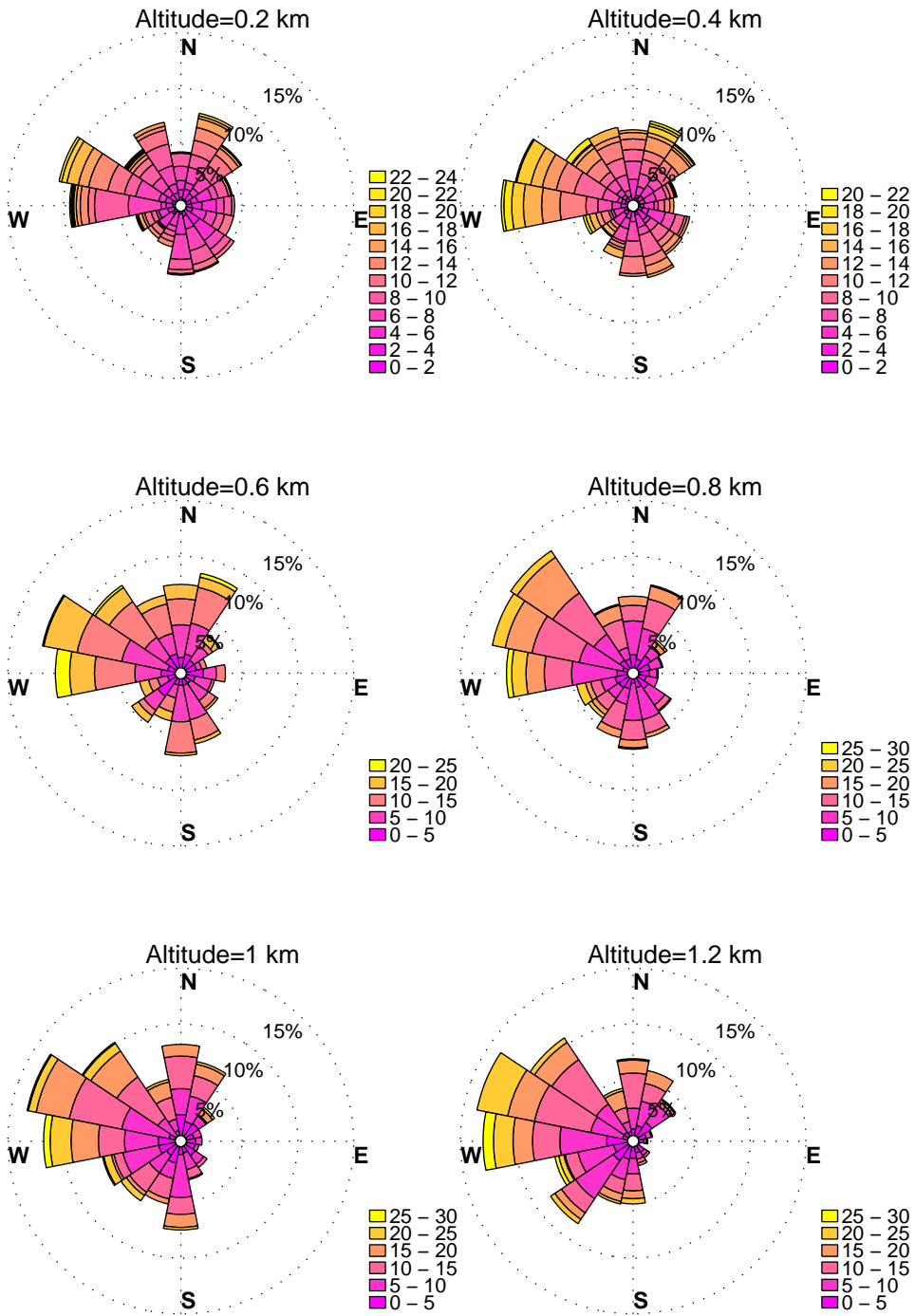
WINDROSES. PINEY RUN, MD WIND PROFILER. SEPTEMBER, HOURS: 12 am to 3 am DATA: FROM 1/2010 to 8/2014
