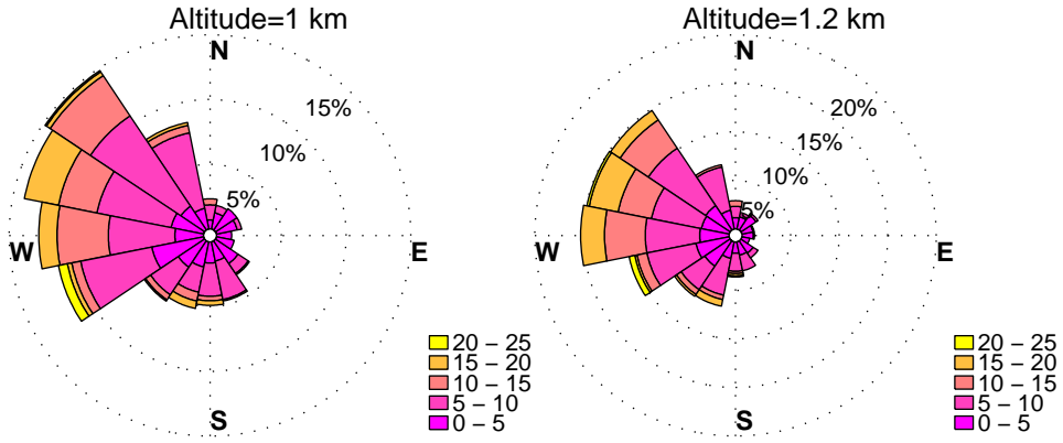
WINDROSES. PINEY RUN, MD WIND PROFILER. SEPTEMBER, HOURS: 12 pm to 15 pm DATA: FROM 1/2010 to 8/2014
