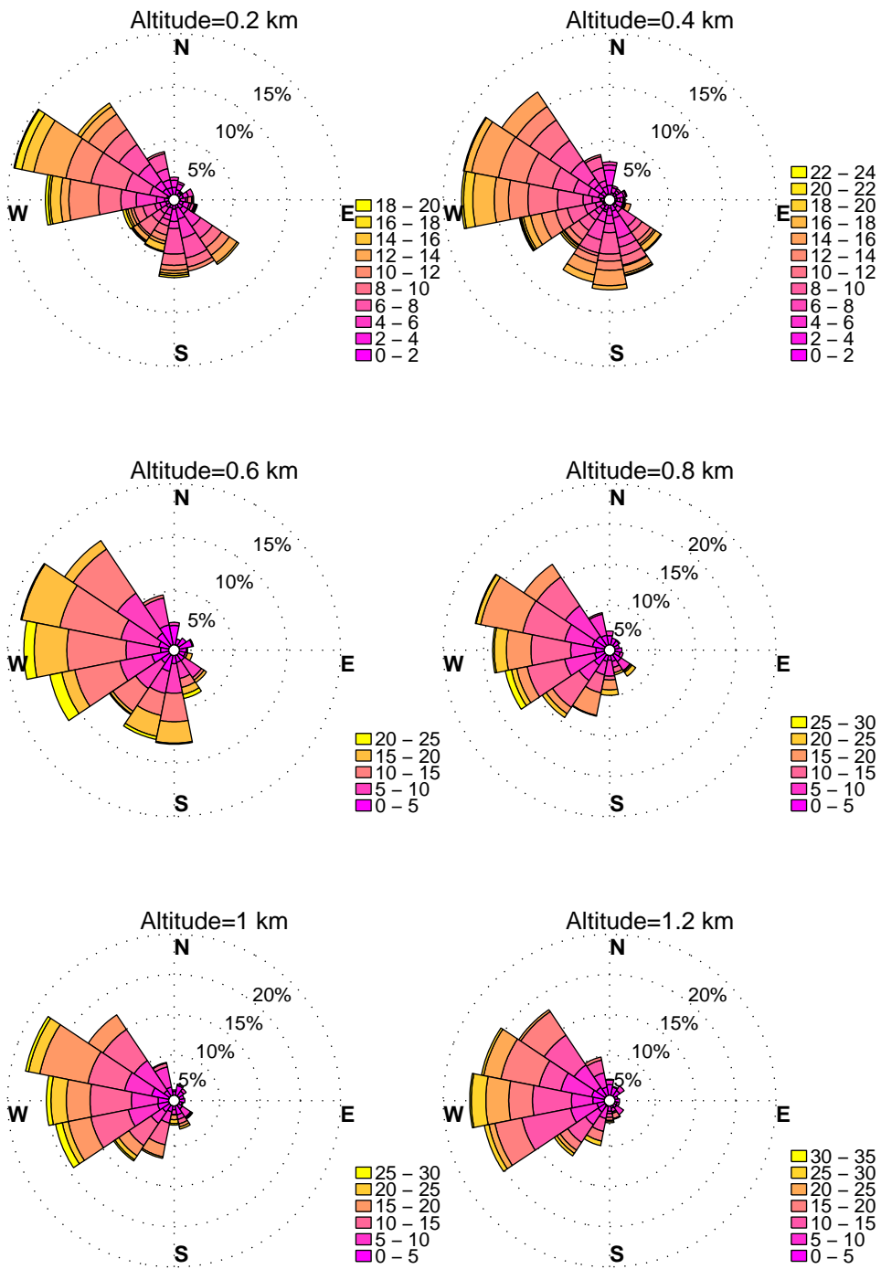
WINDROSES. PINEY RUN, MD WIND PROFILER. APRIL, HOURS: 12 pm to 3 pm DATA: FROM 2010 to 2015
