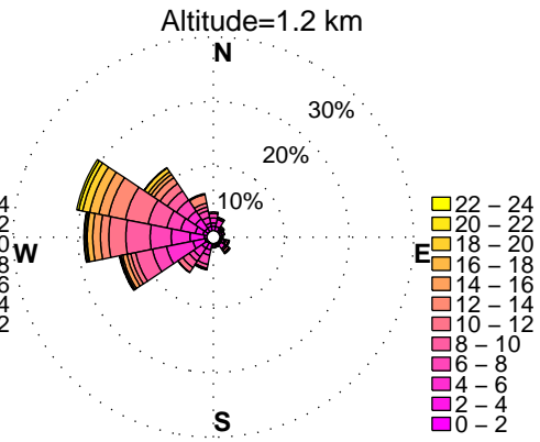
WINDROSES. PINEY RUN, MD WIND PROFILER. AUGUST, HOURS: 12 am to 3 am DATA: FROM 2010 to 2015
